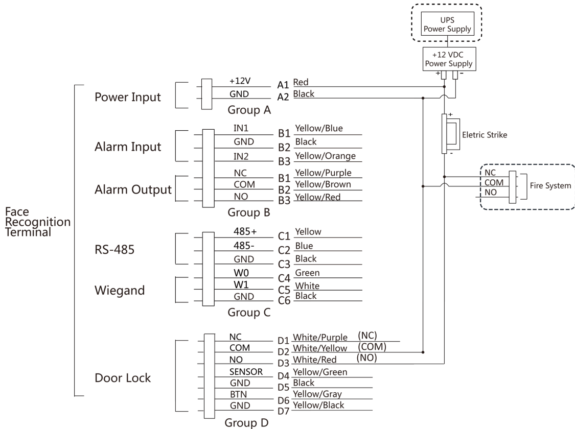
Figure 4-8 Device Wiring
