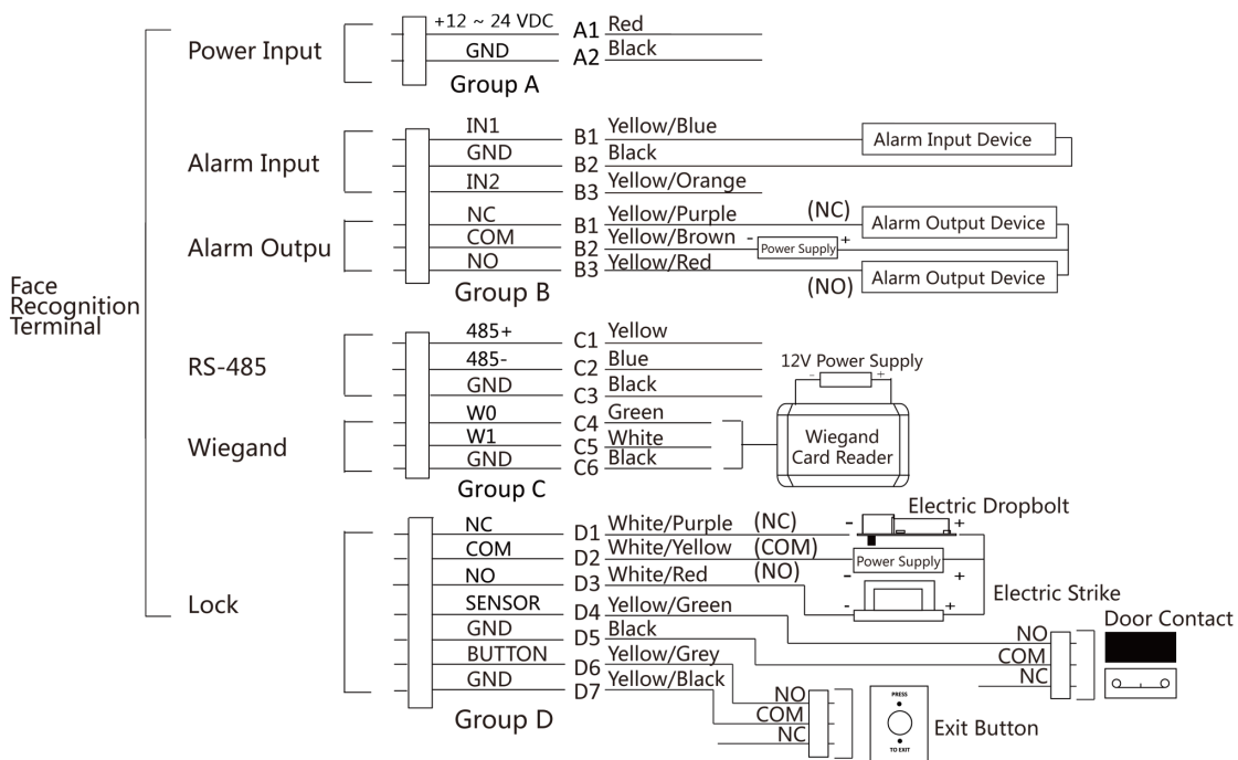
Figure 4-2 Device Wiring
