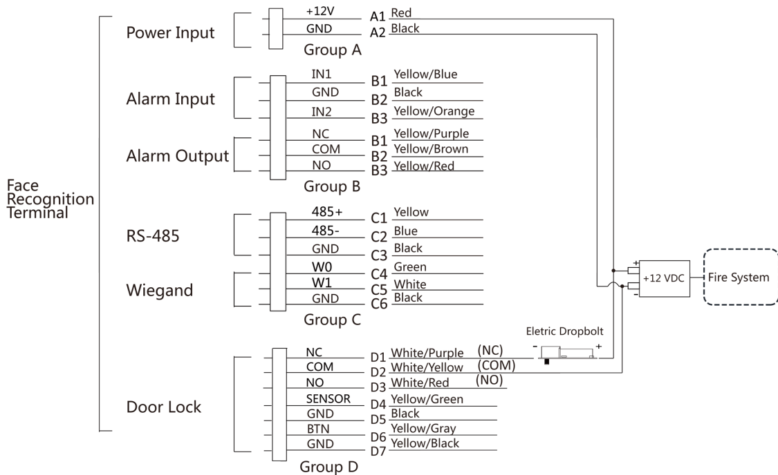
Figure 4-4 Wire Device
