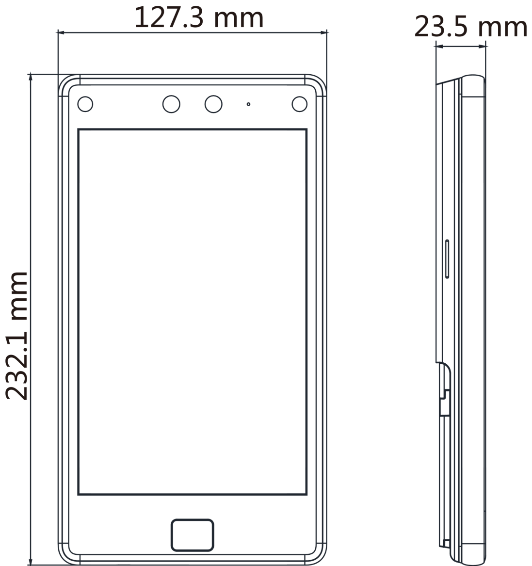
Figure D-1 Dimension
