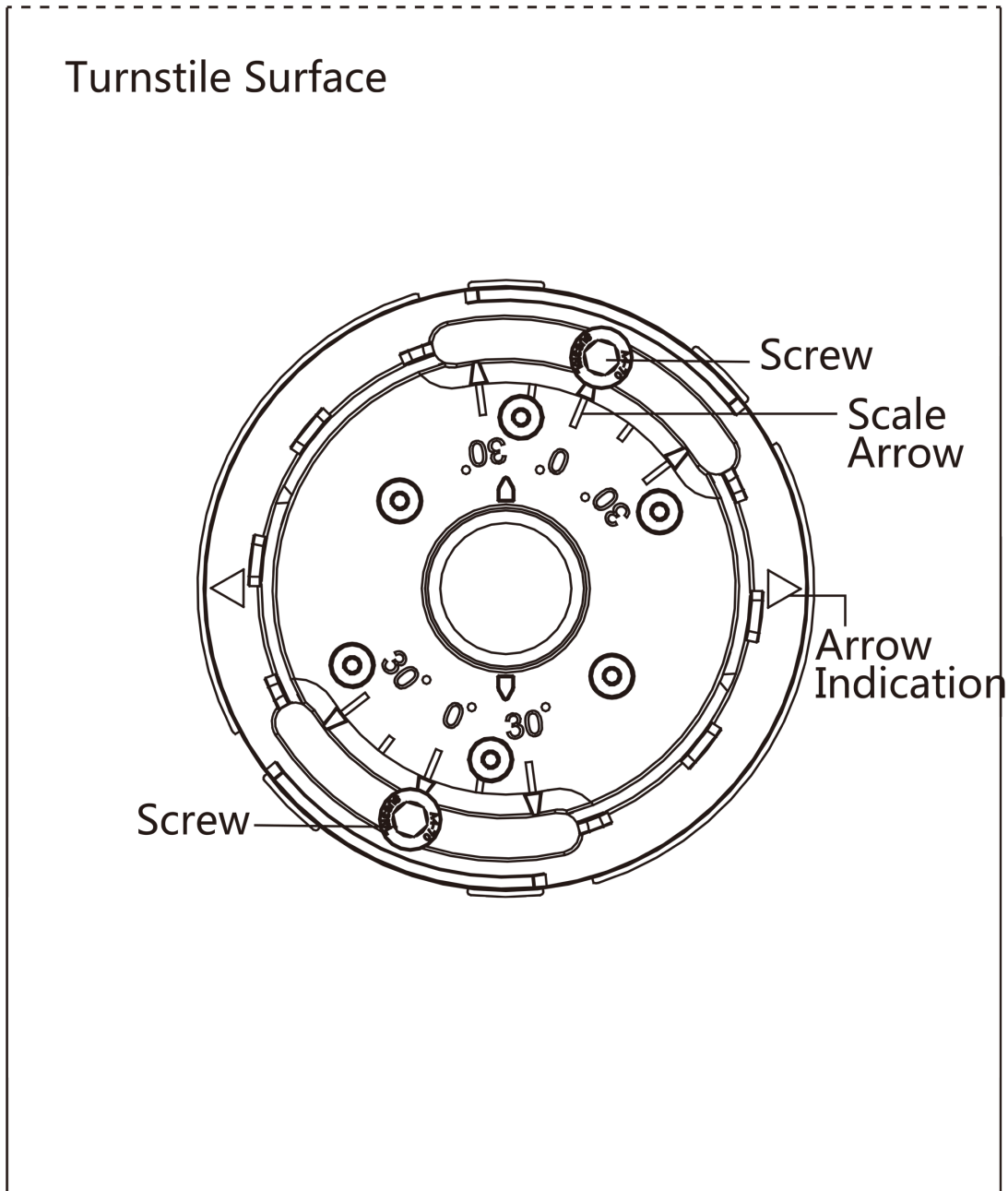
Figure 3-4 Screw Position
