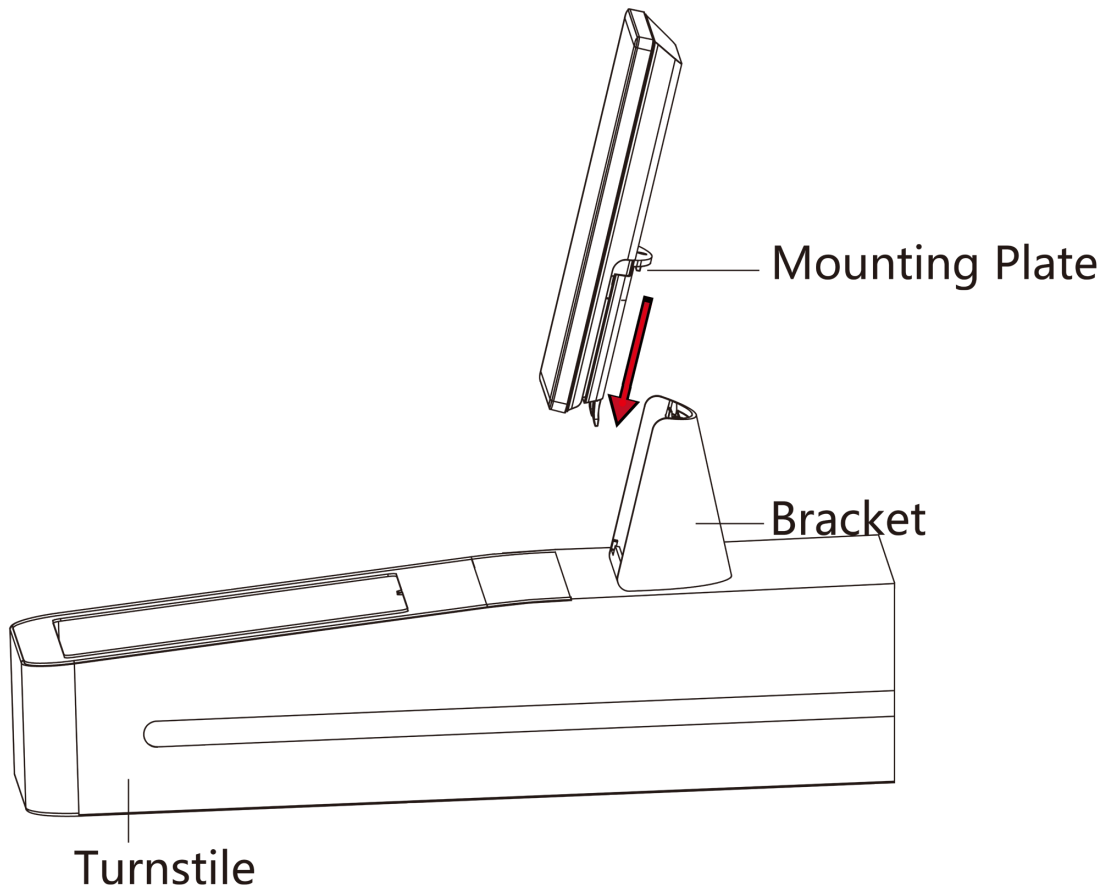
Figure 3-15 Install Device
