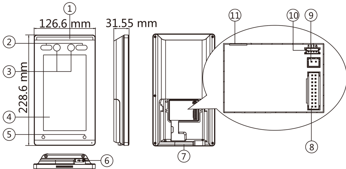
Figure 2-1 Face Recognition Terminal Diagram
