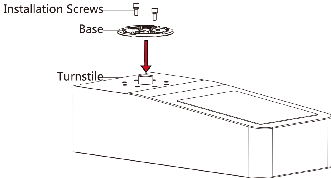
Figure 3-3 Install Base
