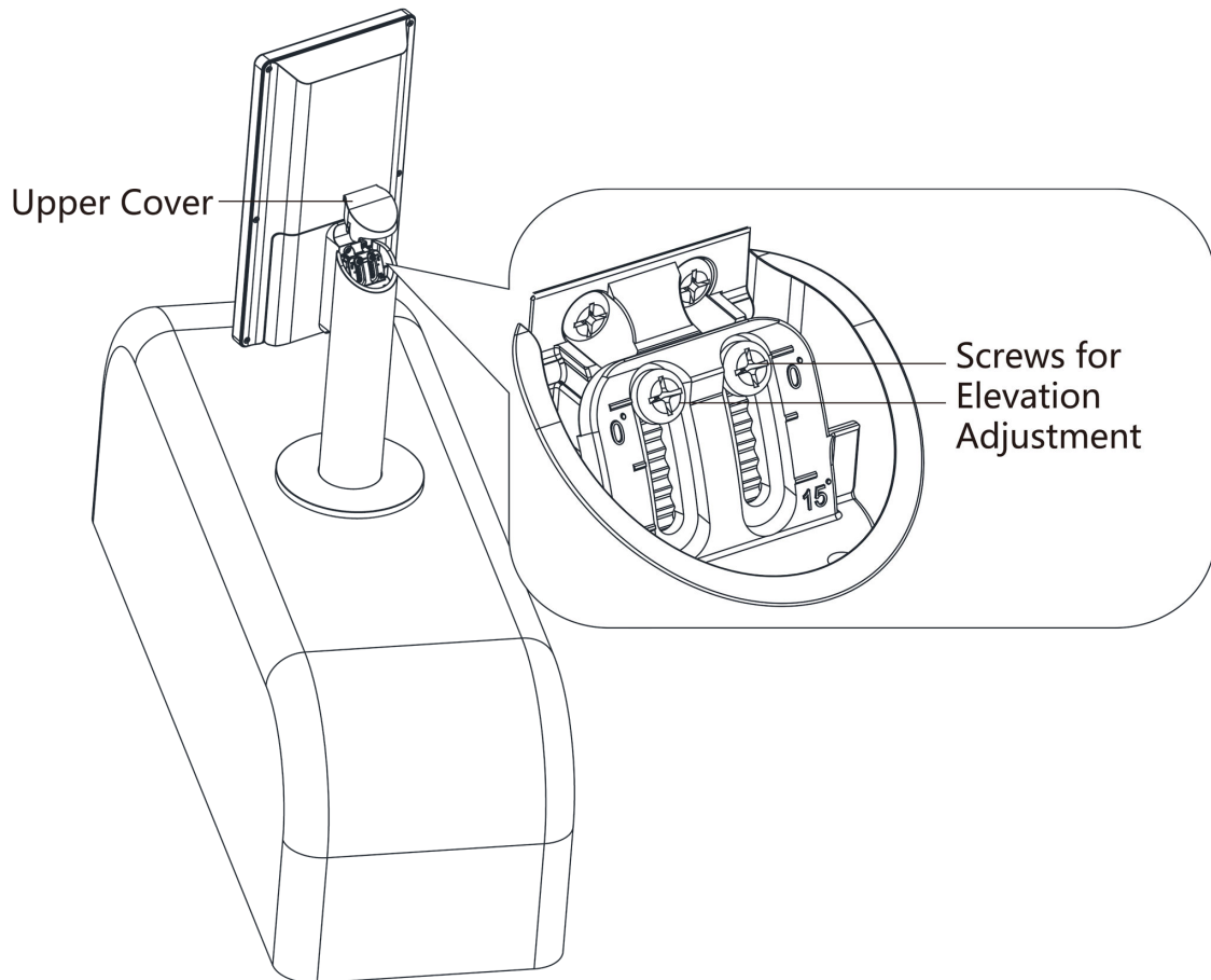
Figure 3-10 Adjust Elevation
