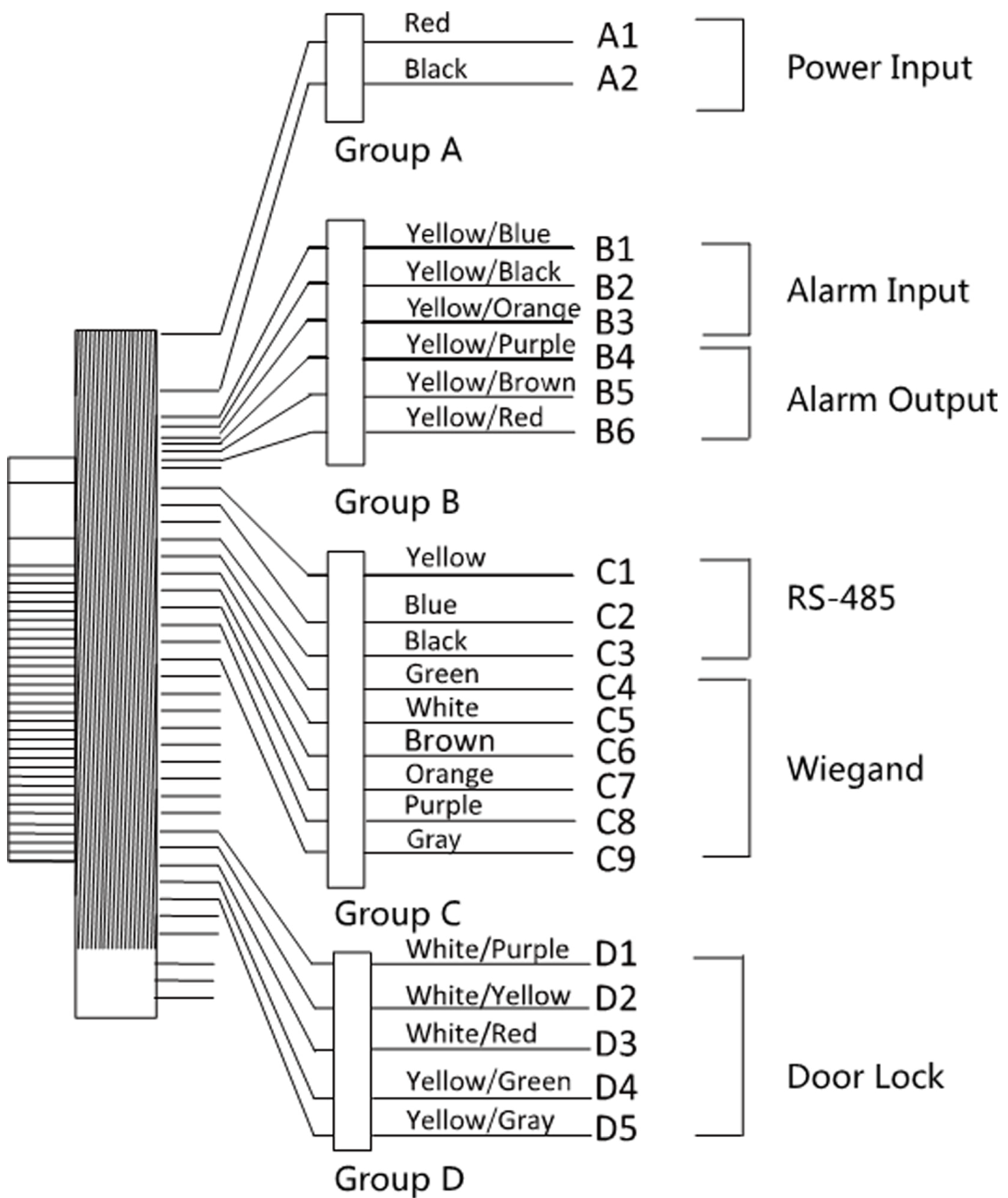
Figure 4-1 Terminal Diagram
