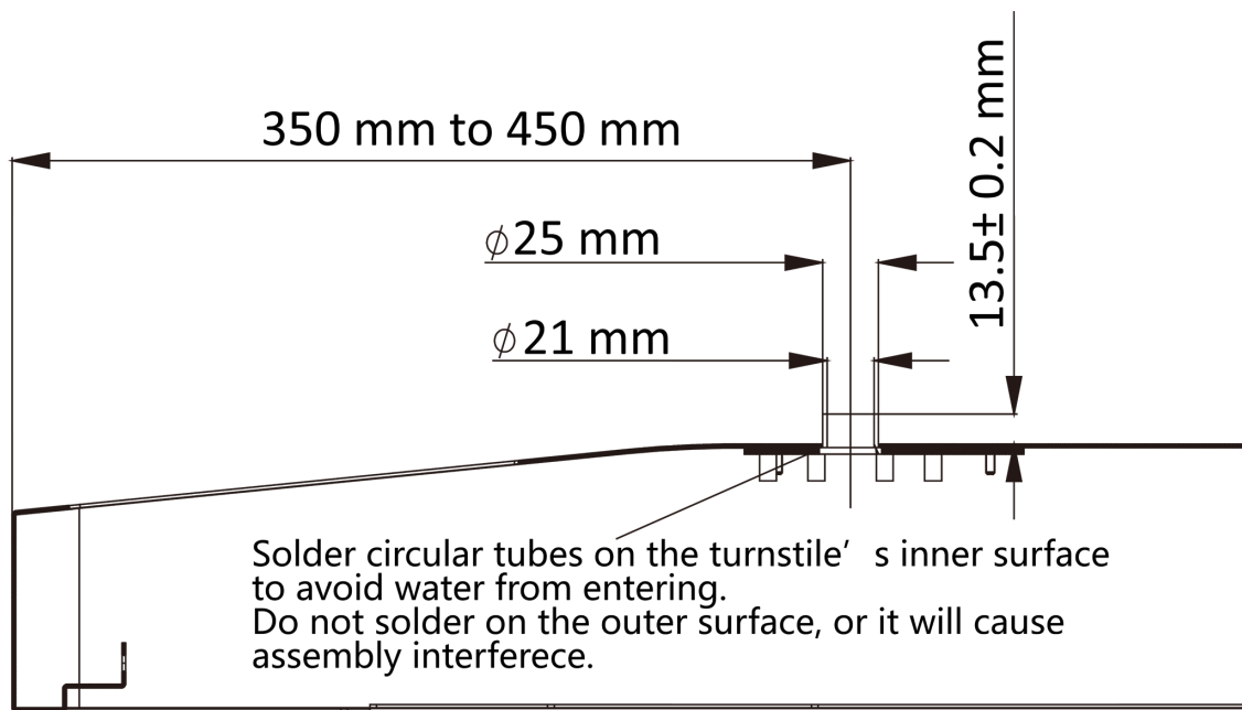
Figure 3-2 Solder Tubes
