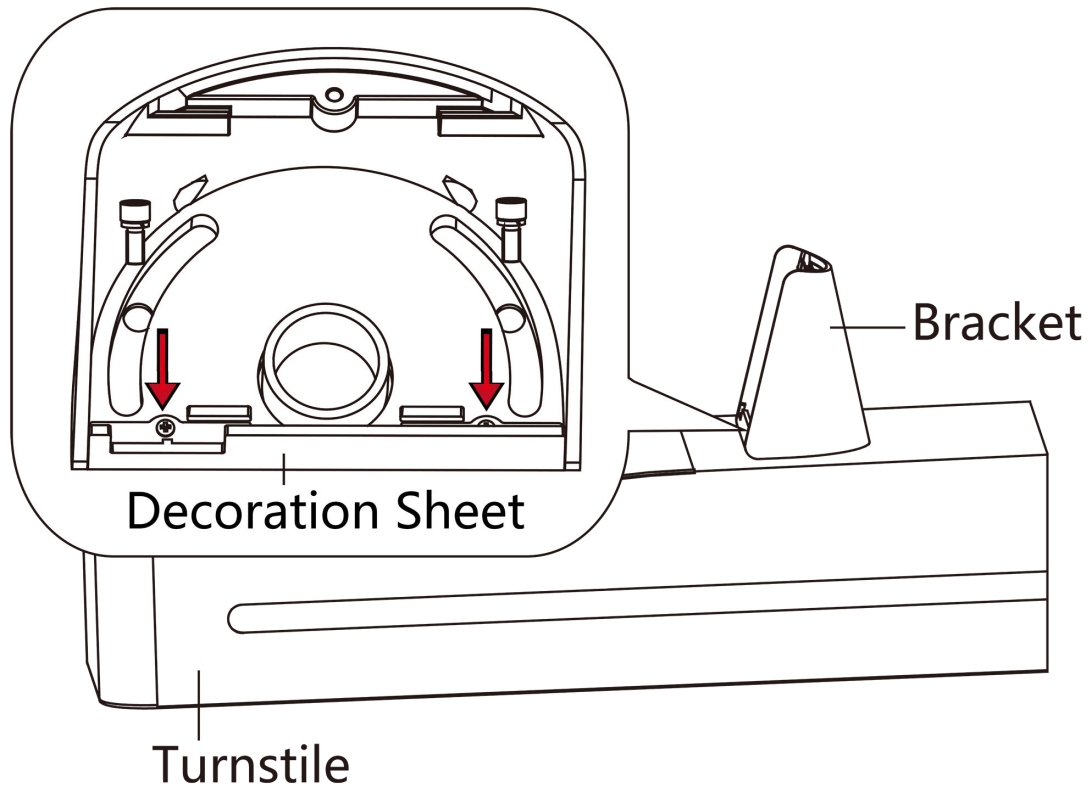
Figure 3-12 Remove Screws
