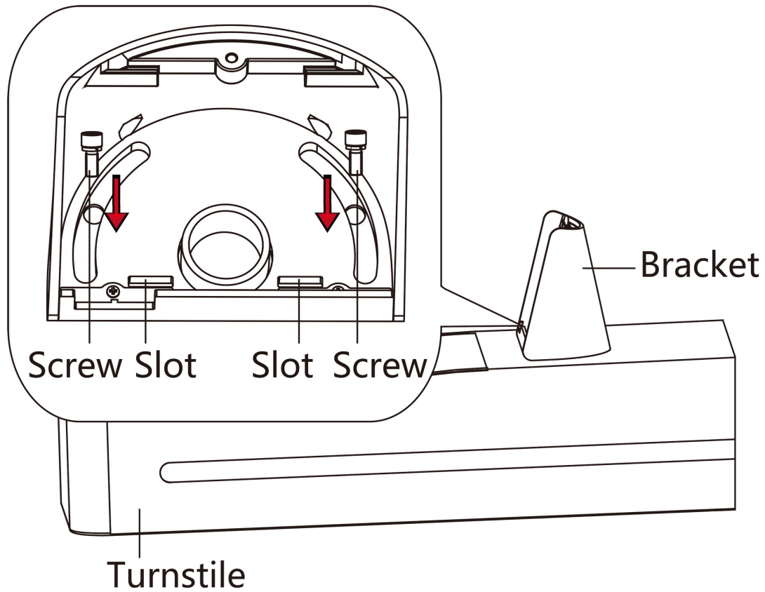
Figure 3-14 Secure Bracket
