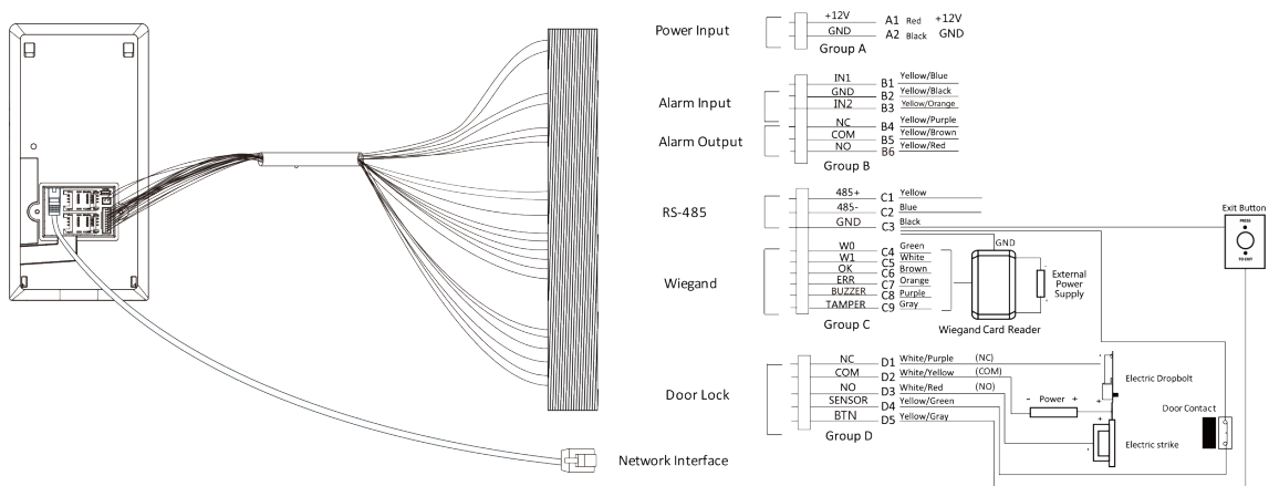
Figure 4-2 Device Wiring
