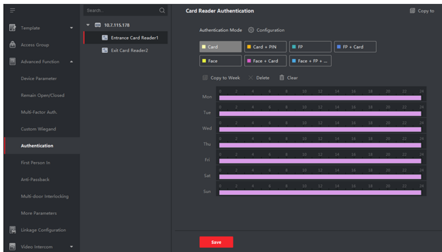
Figure 9-14 Set Authentication Modes for Card Readers
