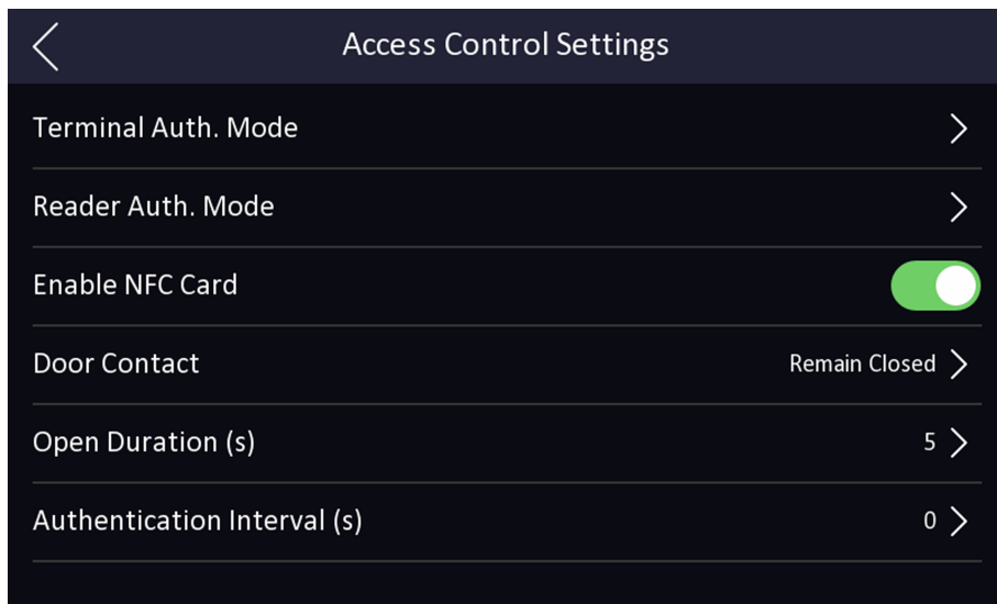
Figure 7-10 Access Control Parameters
