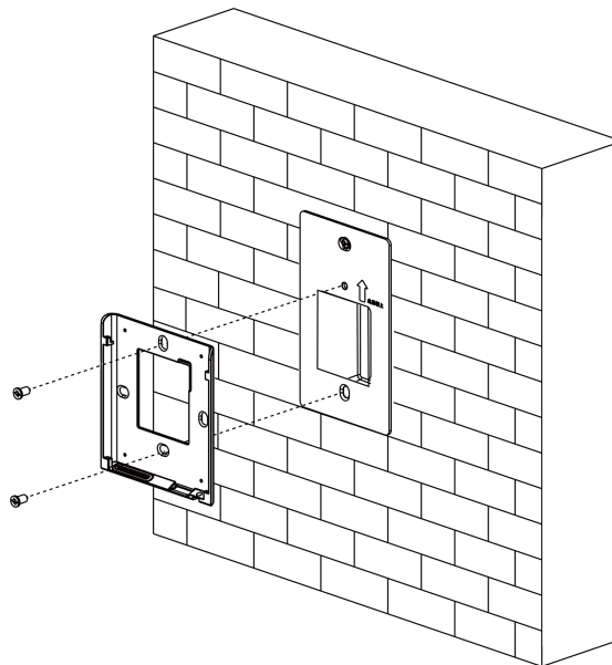
Figure 3-3 Install Mounting Plate
