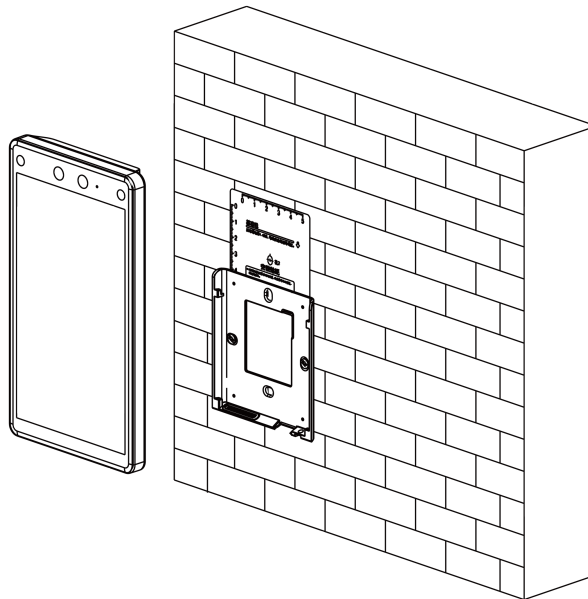
Figure 3-12 Hang Device
