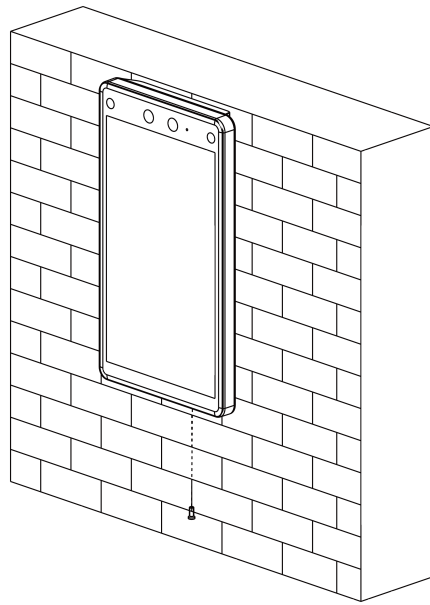
Figure 3-13 Secure Device
