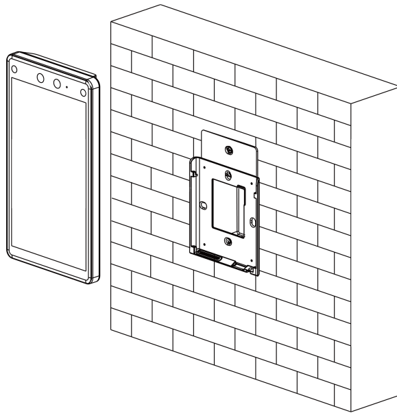
Figure 3-4 Hang Device
