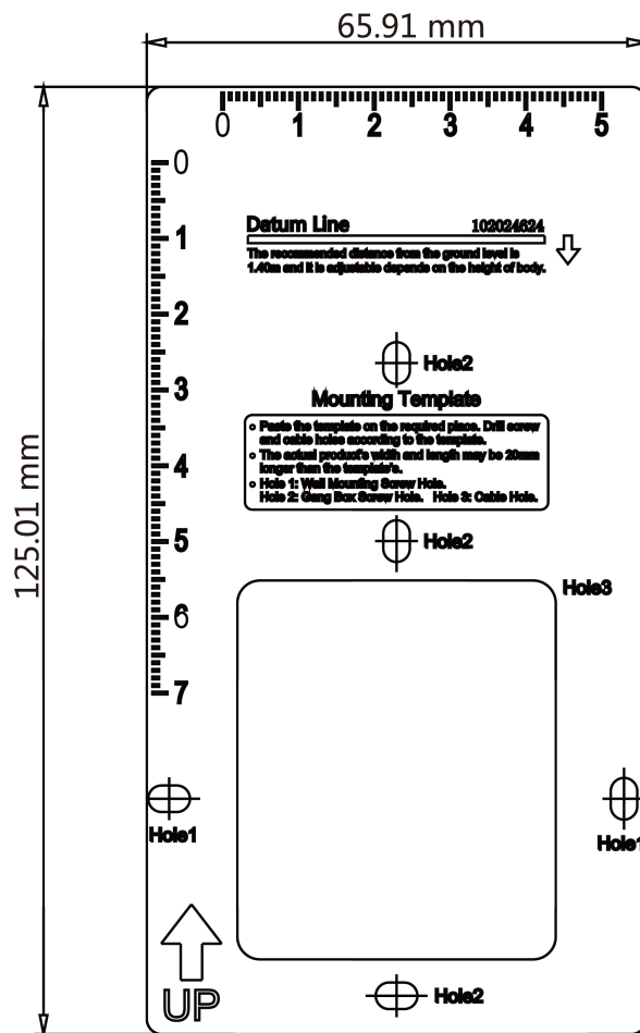
Figure 3-10 Mounting Template
