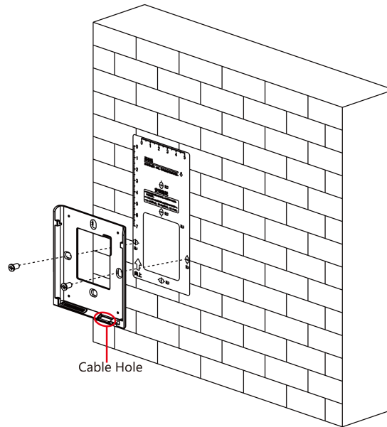
Figure 3-11 Install Mounting Plate
