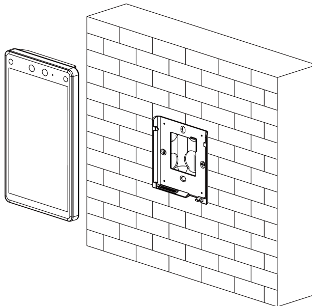
Figure 3-8 Hang Device
