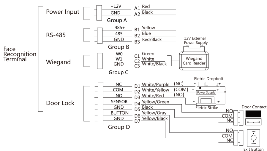
Figure 4-1 Device Wiring
