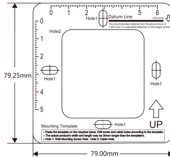
Figure 3-1 Mounting Template
