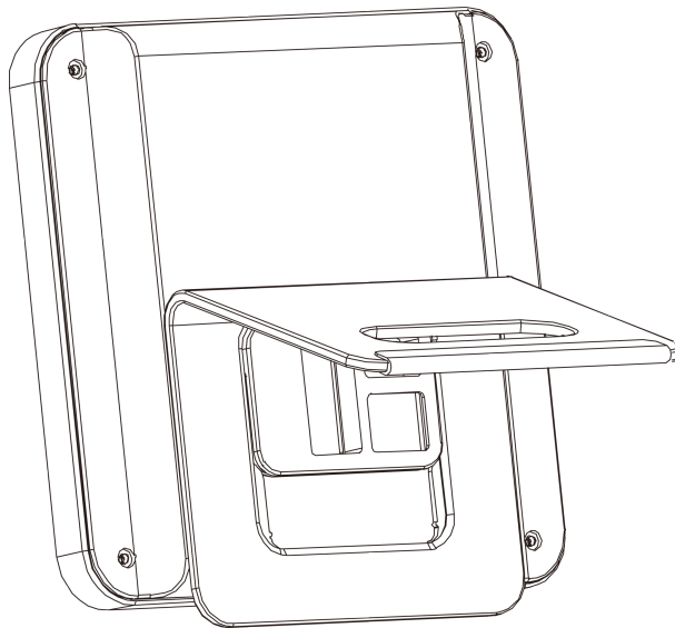
Figure 3-5 Align Bracket and Device
