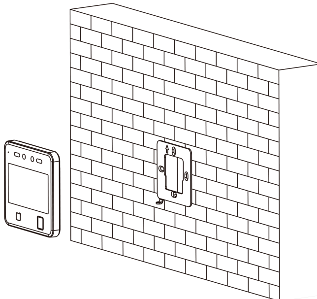
Figure 3-3 Hang Device
