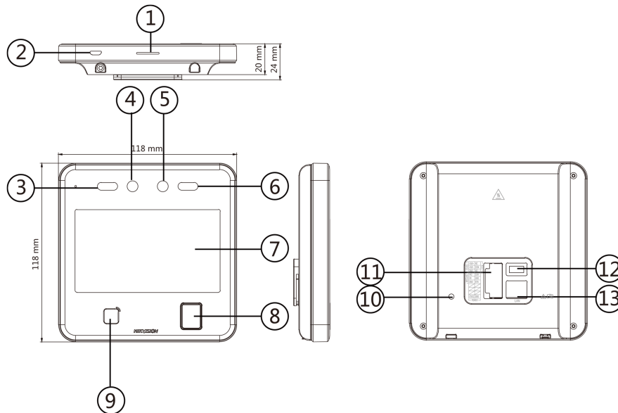
Figure 2-1 Face Recognition Terminal Diagram
